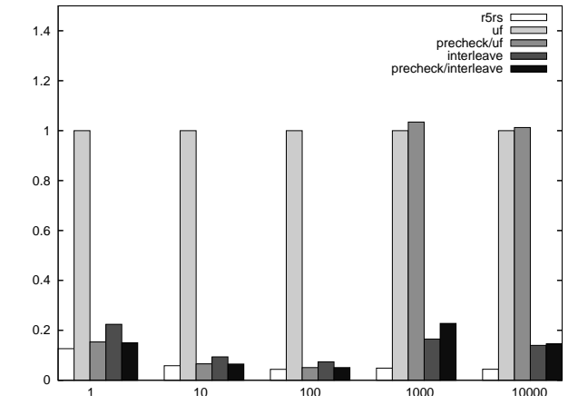
Figure 9. Inverted lists of various lengths
