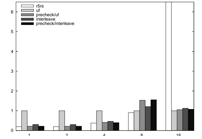
Figure 12. Random dags
