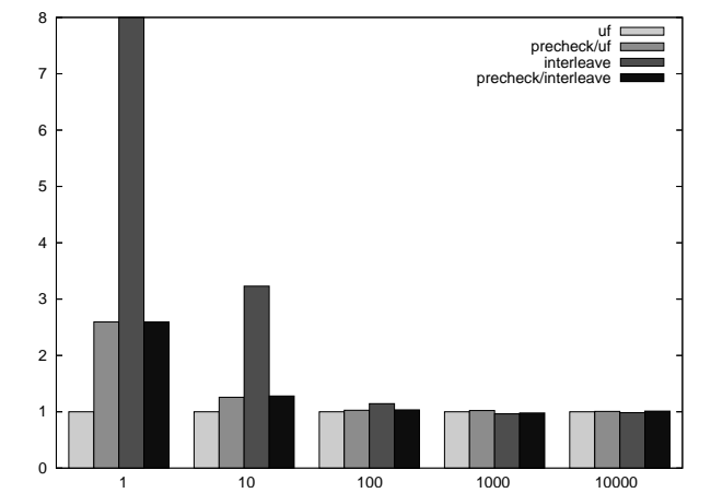
Figure 14. Union-exercising graphs
