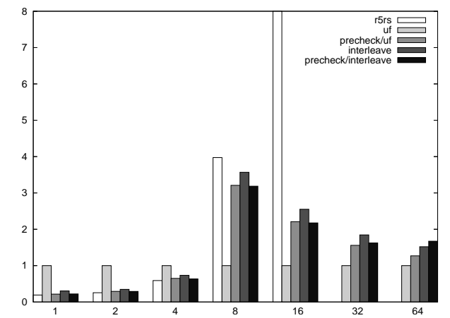
Figure 11. Degenerate dags
