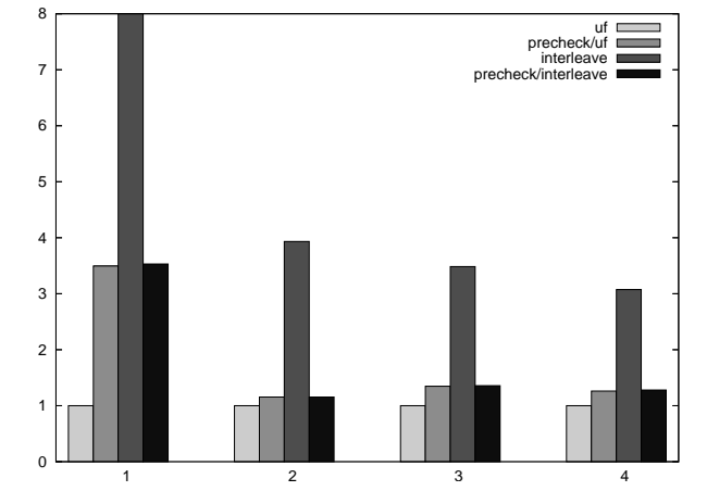
Figure 13. Random graphs
